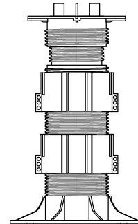
LC + C4 + C4 RANGO VERTICAL: 8 3/4" - 12" (222mm - 305mm)
