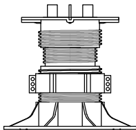
LC + C1 RANGO VERTICAL: 4 3/4" - 6 1/4" (121mm - 159mm)
