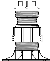
LC + C4 RANGO VERTICAL: 6 1/4" - 8 3/4" (159mm - 222mm)
